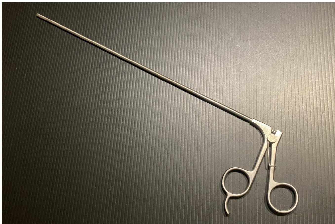
Jarrit Biopsy Forceps, 1x1 Teeth, 5mm, 330mm 11.5mm jaw
